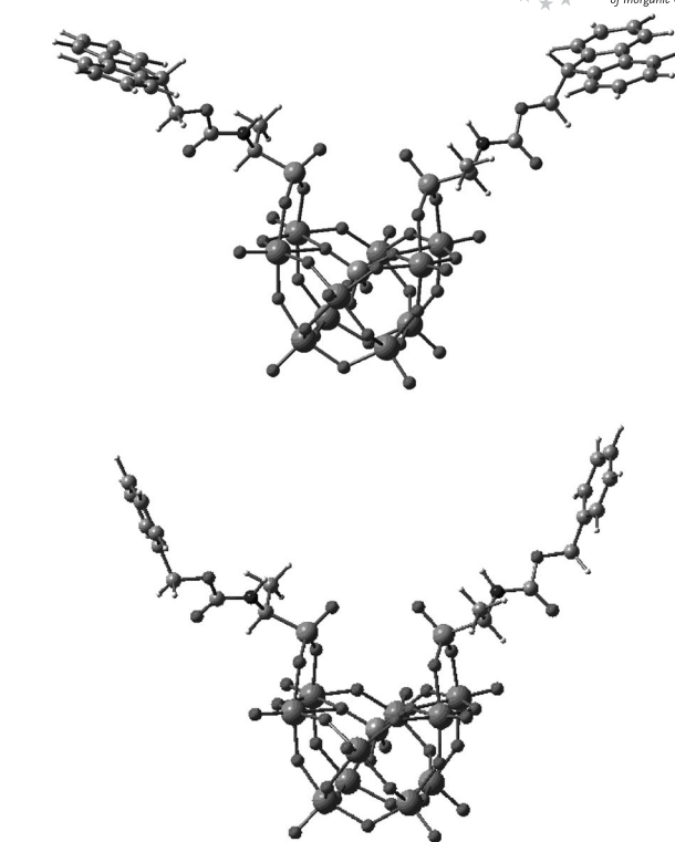
Figure 3. Optimized geometries of 1 (top) and 2 (bottom).
